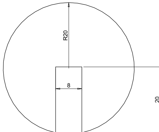
DETAIL A - FRONT VIEW
